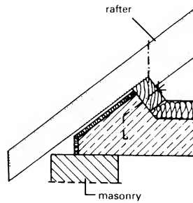
5 Rafter continued to the eaves
